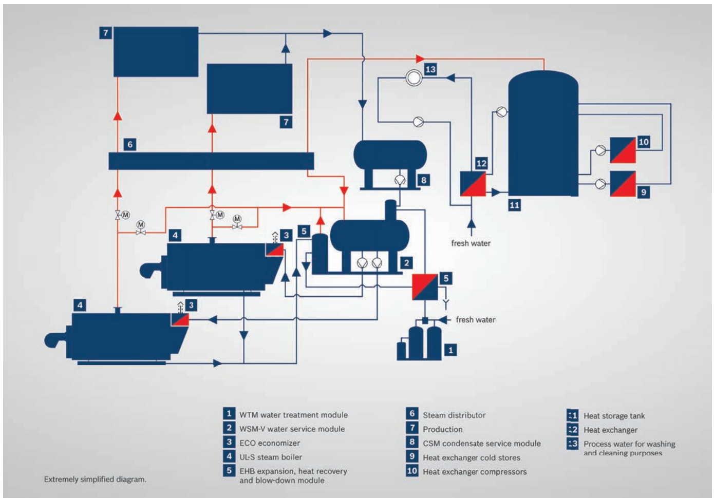
System diagram steam boiler with appropriate plant technology for heat recovery, water treatment and waste heat utilisation involving the compressors and cold stores
