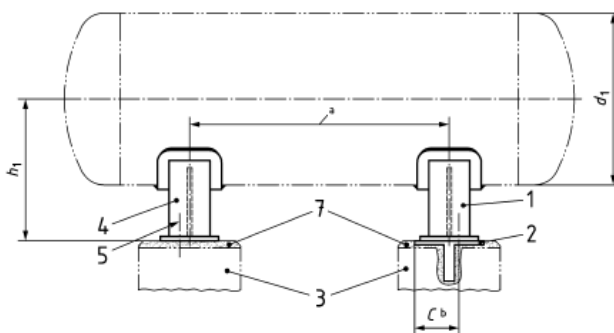
Installation on foundations
