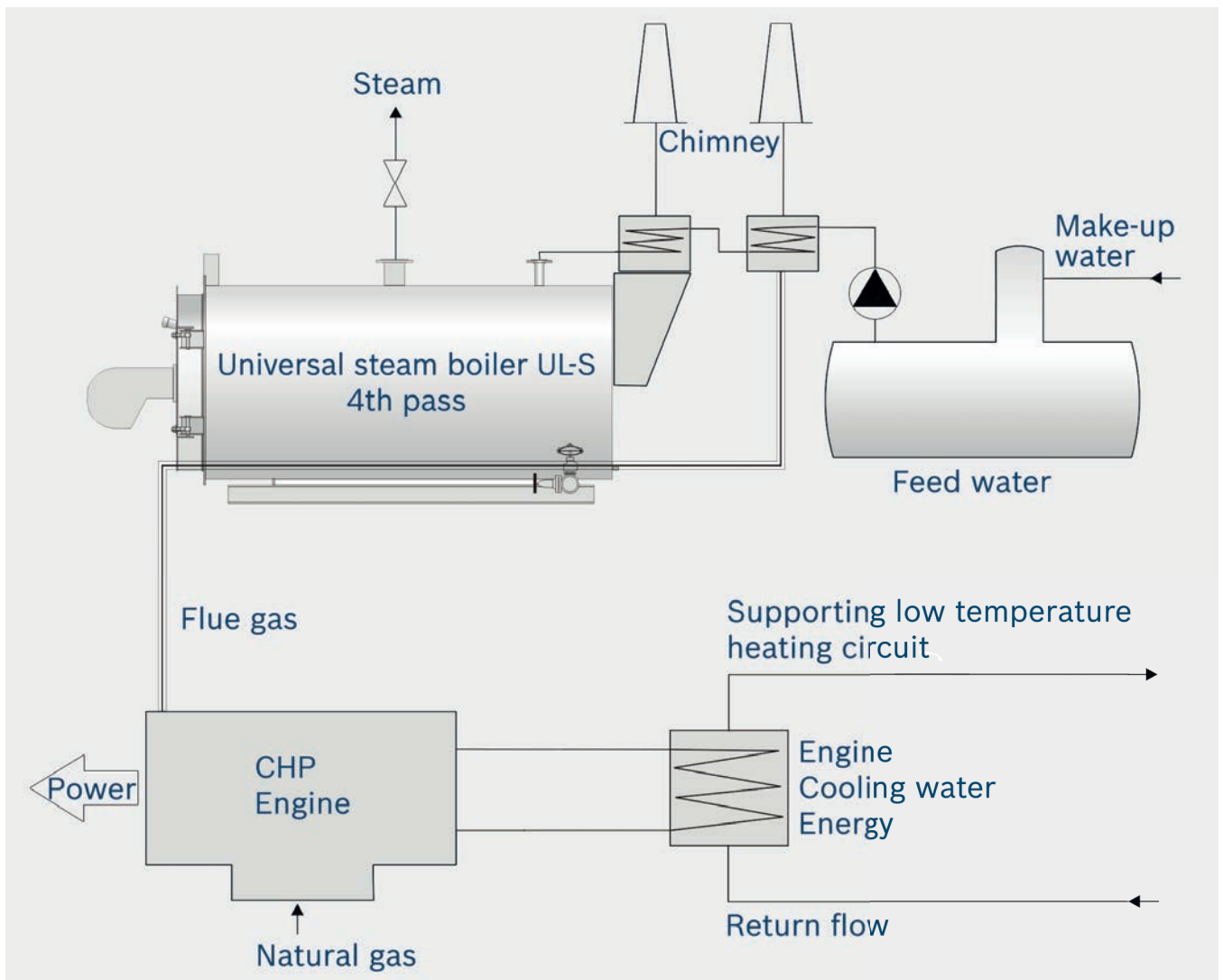
System diagram of CHP unit and self-fired four-pass boiler combination at Immergut
